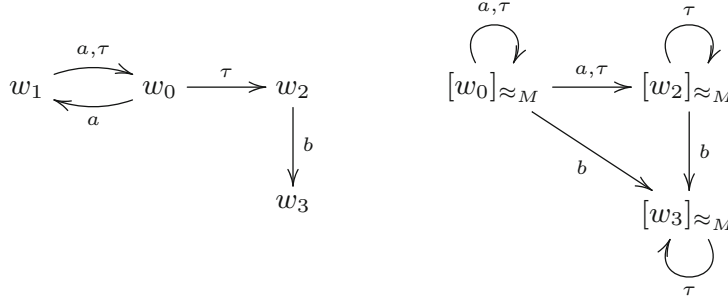
Fig. 3. A structure M and its quotient M/\approx_M
